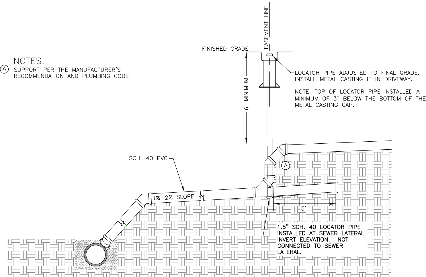
RECOMMENDED SEWER SERVICE INSTALLATION METHOD #2 NOT TO SCALE
