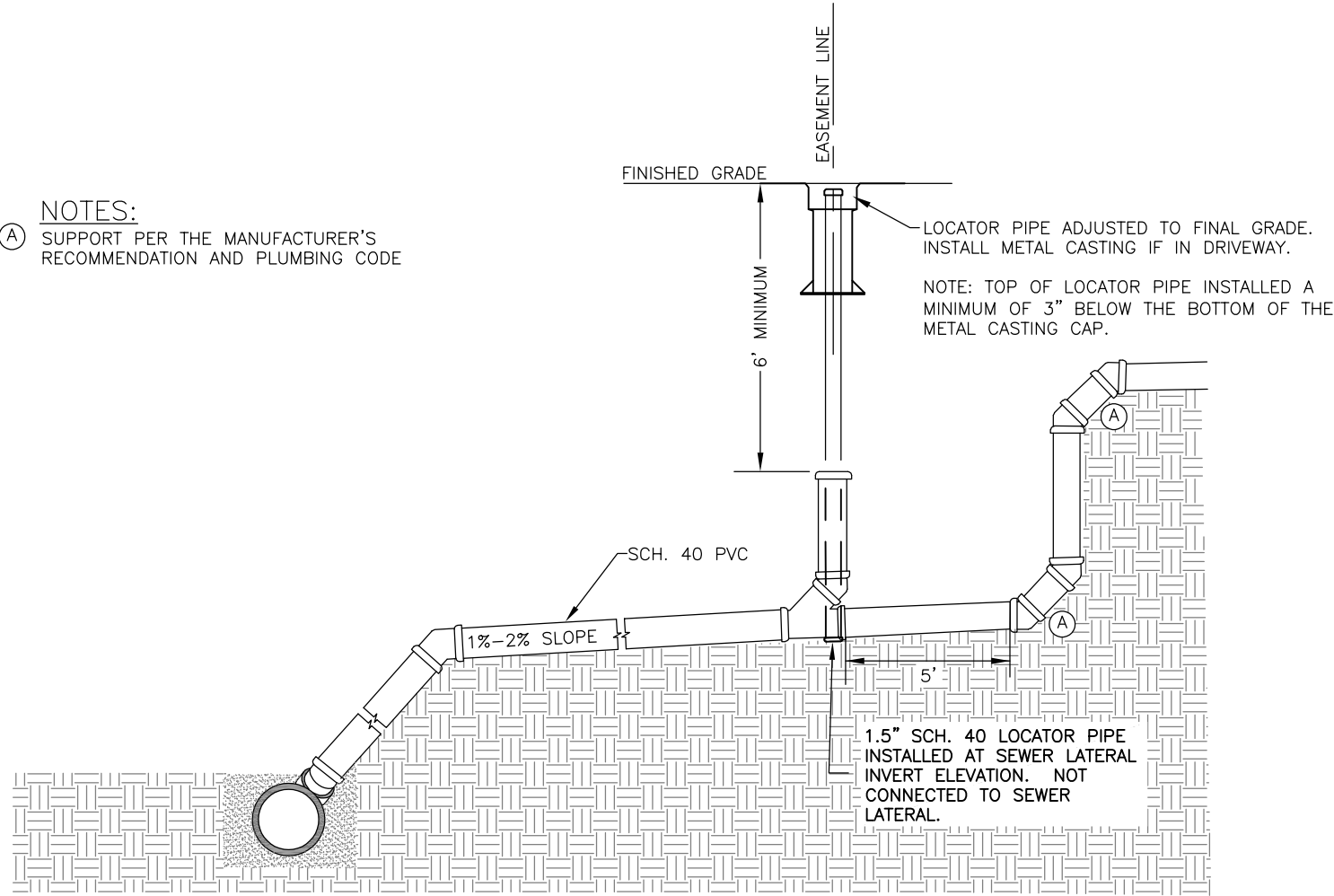
RECOMMENDED SEWER SERVICE INSTALLATION METHOD #1 NOT TO SCALE
